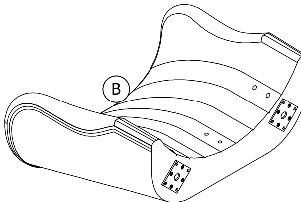
Back X 1
