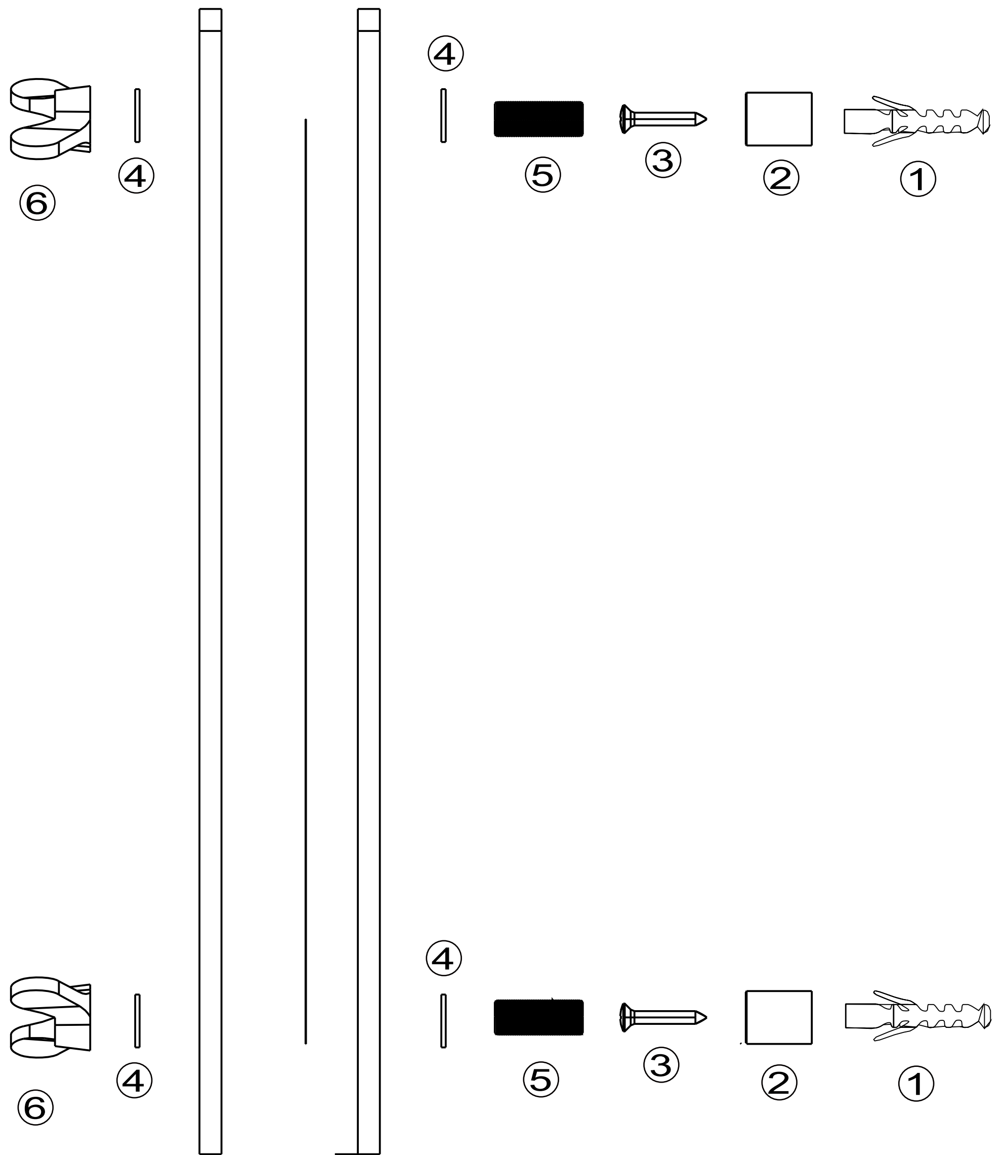
Assembly sequence of nails
